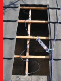
TILED ROOF
